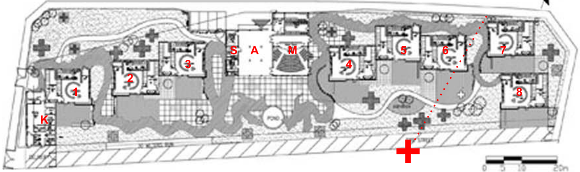
SITE SNAPSHOT 03, 2009.11.10.Tue ROOF TOPPING BLDS. 6-8 SITE PLAN WITH LOCATTION OF SNAPSHOT +
